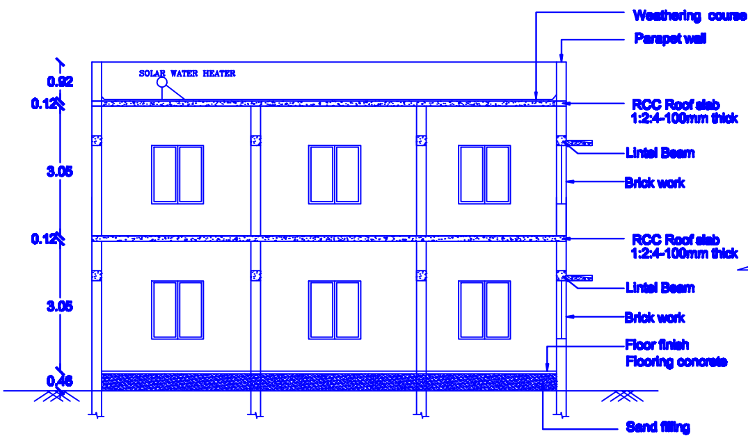
SECTION -XY
