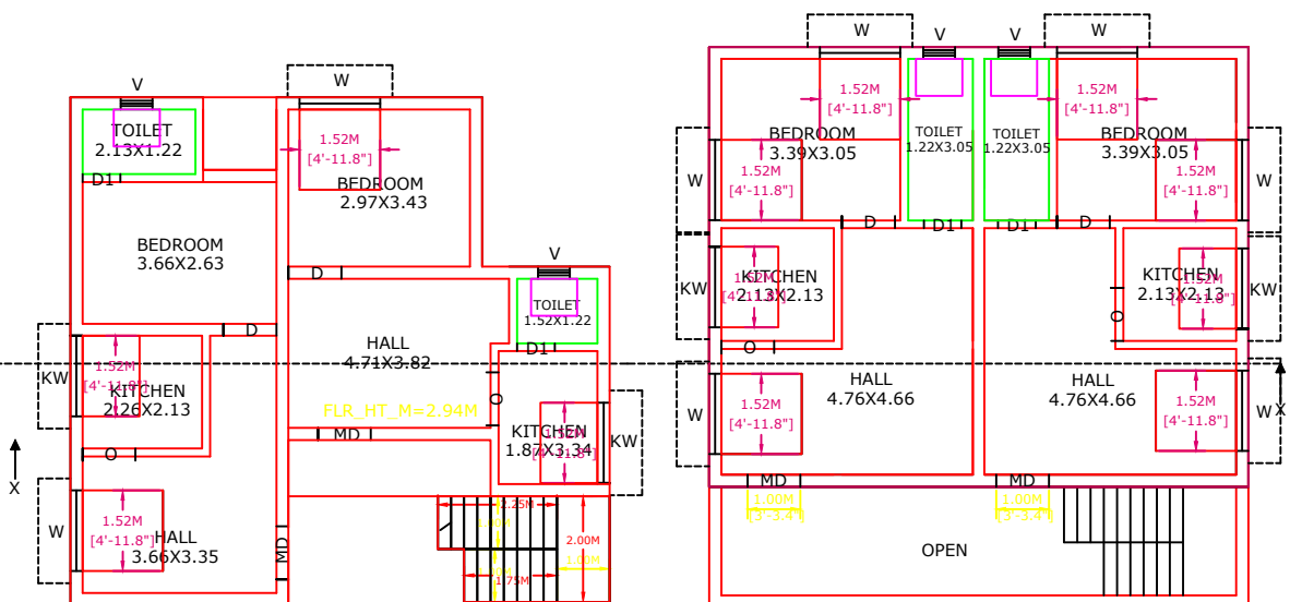
EXI. GROUND FLOOR PLAN
