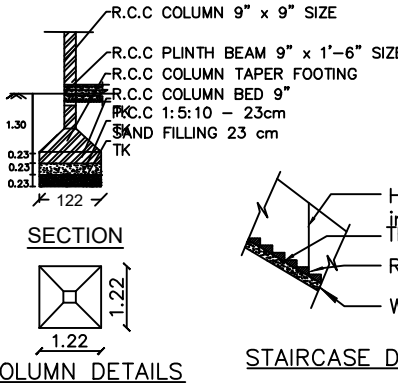
COLUMN DETAILS
