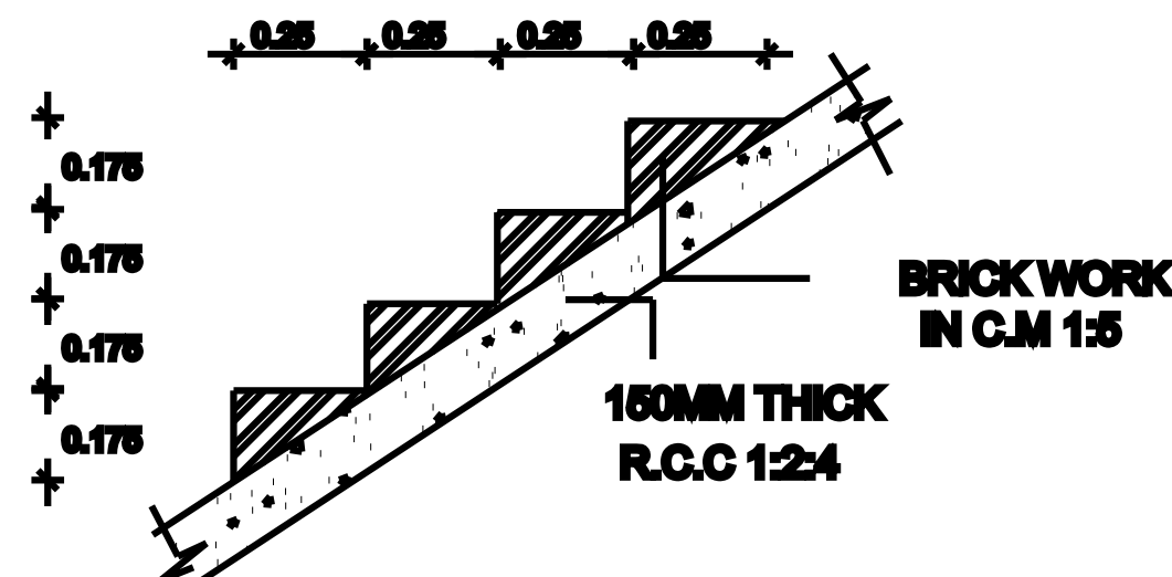
STAIRCASE DETAILS NOT TO SCALE
