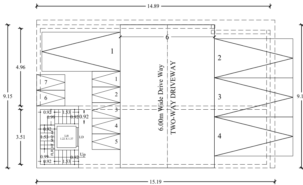
STILT FLOOR PLAN
