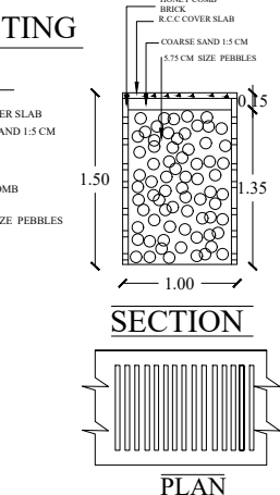
RAIN WATER HARVESTING PERCOLATION BED
