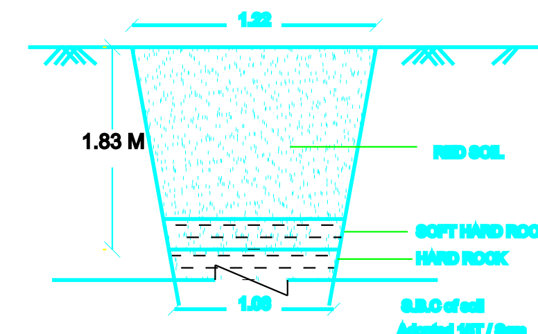
TRIAL PIT DETAILS NOT TO SCALE
