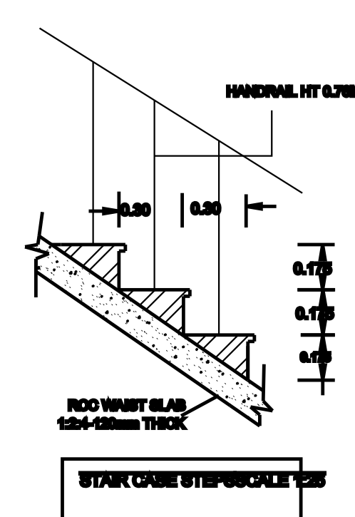
STAIR CASE STEP SCALE
