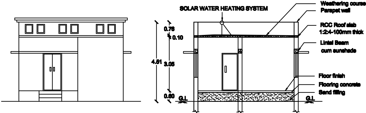
FRONT ELEVATION
