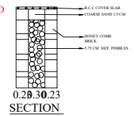
SECTION PLAN
