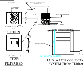
RAIN WATER COLLECTION SYSTEM FROM TERRACE
