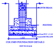
COLUMN FOUNDATION DETAILS NOT TO SCALE
