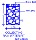
COLLECTING RAIN WATER PIT Not to Scale
