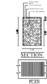
RAIN WATER HARVESTING PERCOLATION BED
