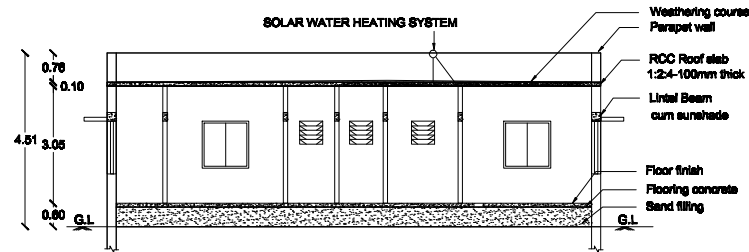
SECTION ON MK
