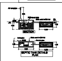
WATER TANK DETAILS SCALE 1:50
