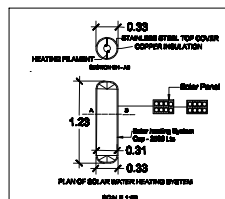
PLAN OF SOLAR WATER HEATING SYSTEM SCALE 1:50
