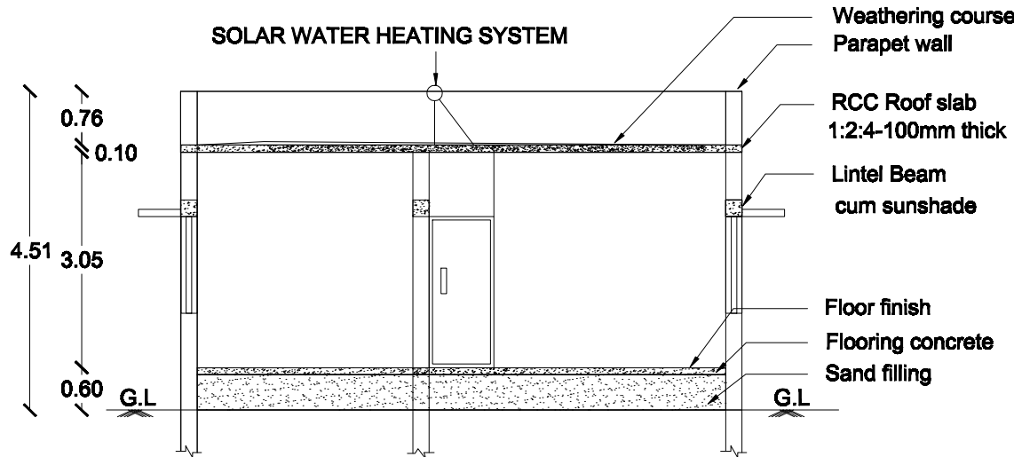
SECTION ON MK
