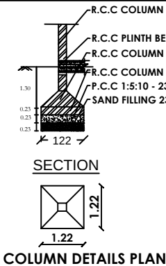
COLUMN DETAILS PLAN
