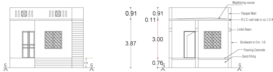
FRONT ELEVATION
