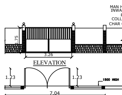
PLAN Compound wall Detail
