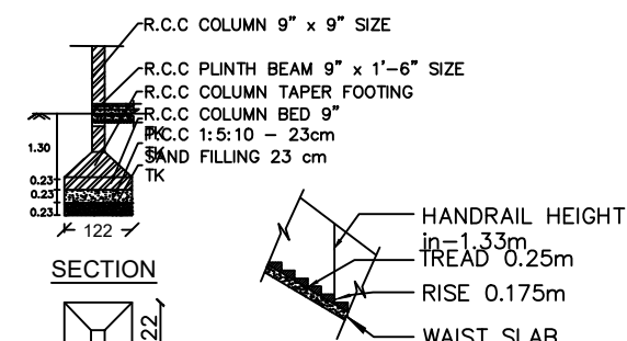
COLUMN DETAILS PLAN
