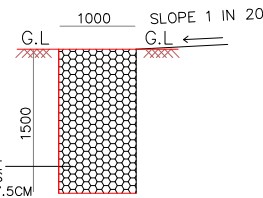
SECTION OF PEBBLE TRENCH SCALE : 1: = 100
