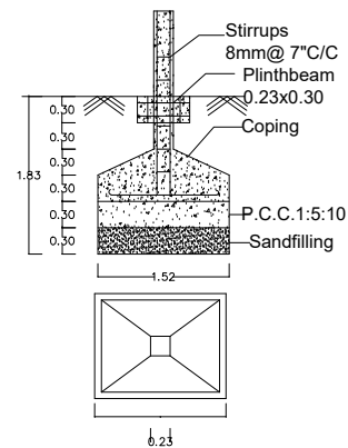
Foundation Details
