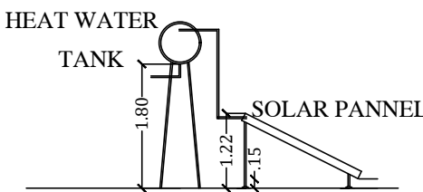
SIDE ELEVATION
