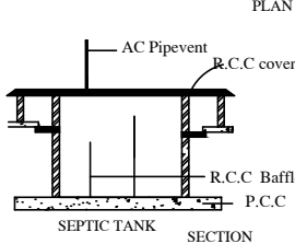
SEPTIC TANK SECTION NOT TO SCALE
