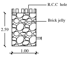
COLLECTING RAIN WATER PIT Not to Scale
