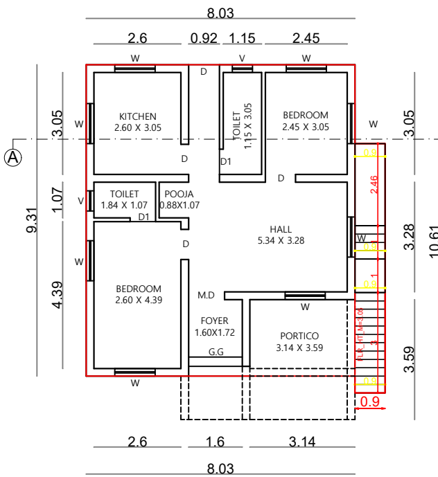
EXI. GROUND FLOOR PLAN
