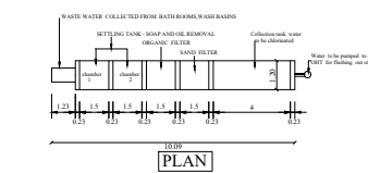
WASTE WATER RECYCLING SYSTEM
