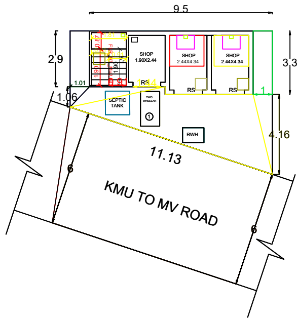
GROUND FLOOR & SITE PLAN
