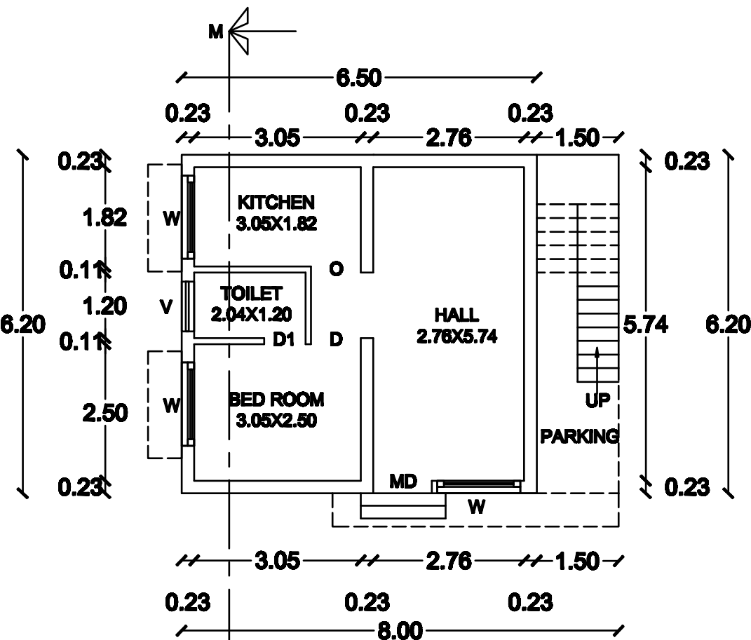
EXG - GROUND FLOOR PLAN
