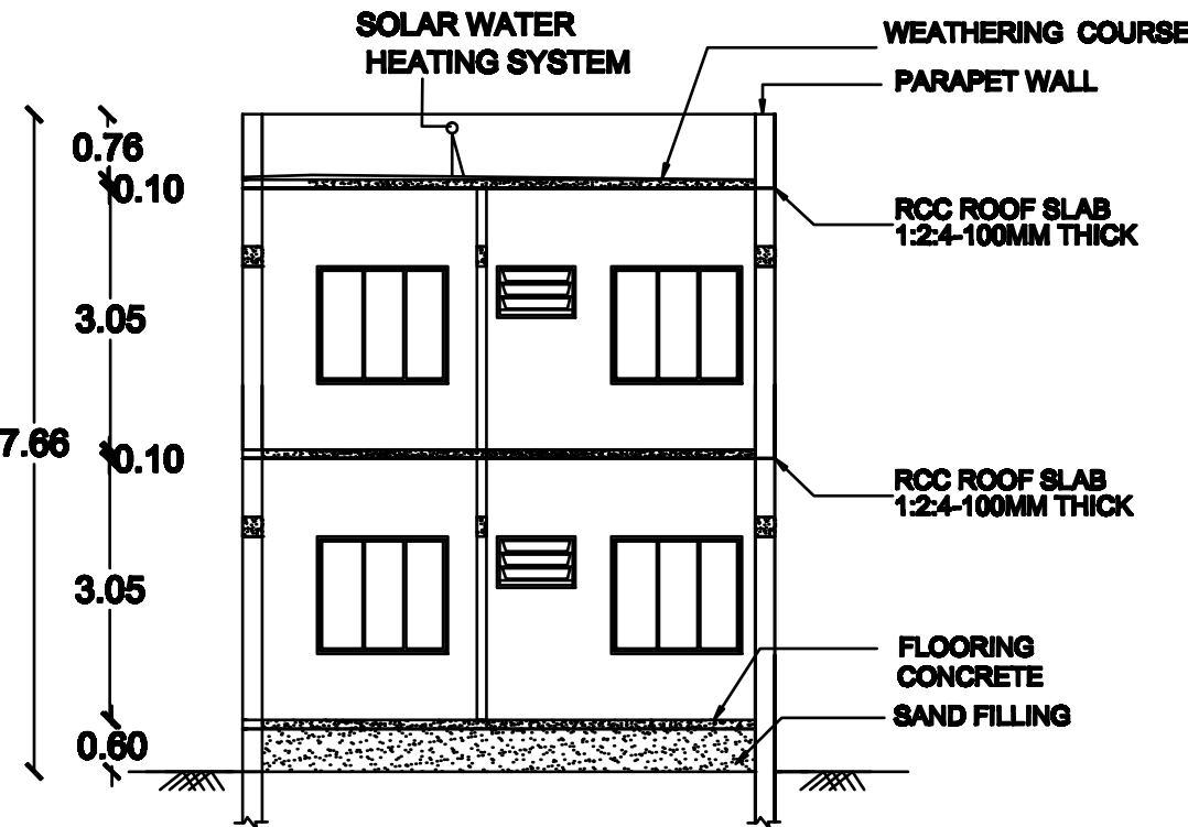
SECTION ON RM
