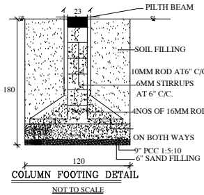
COLUMN FOOTING DETAIL
