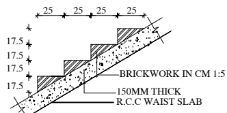
DETAIL OF THE STEPS
