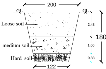
Trail pit details
