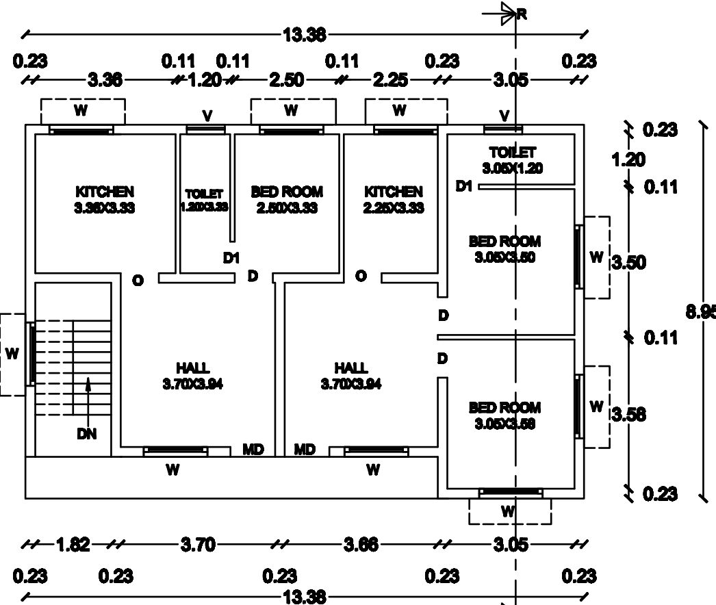
PRO - FIRST FLOOR PLAN
