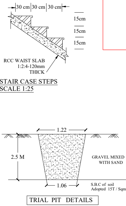
TRIAL PIT DETAILS
