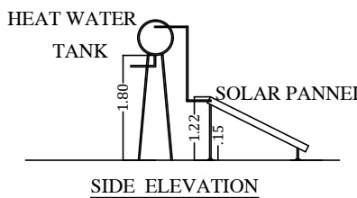
SIDE ELEVATION
