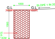
SECTION OF PEBBLE TRENCH SCALE : 1 : 100
