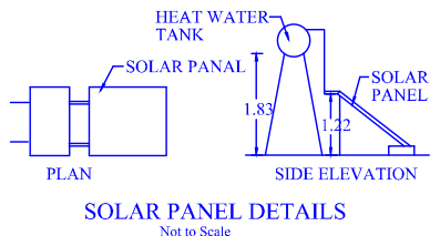
SOLAR PANEL DETAILS Not to Scale
