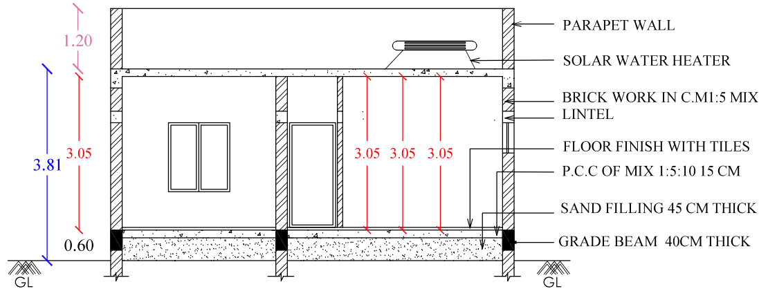
SECTION ON A-A1
