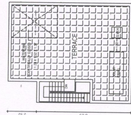
TERRACE PLAN
