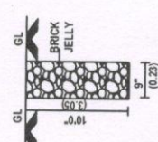
PERCOLATION PIT
