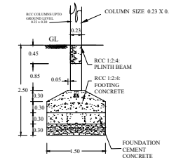
FOUNDATION DETAILS Scale 1:50
