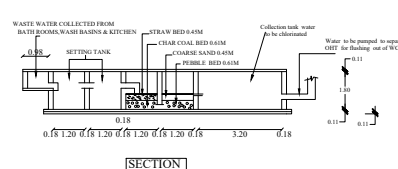
WASTE WATER RECYCLING SYSTEM
