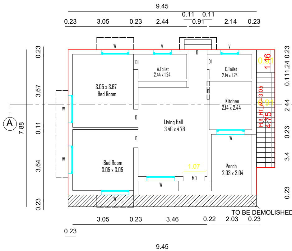
EXI. GROUND FLOOR PLAN
