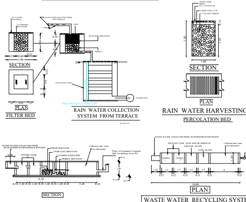
WASTE WATER RECYCLING SYSTEM
