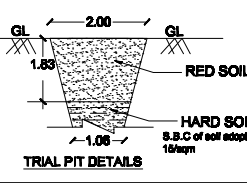
TRIAL PIT DETAILS
