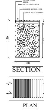
RAIN WATER HARVESTING PERCOLATION BED
