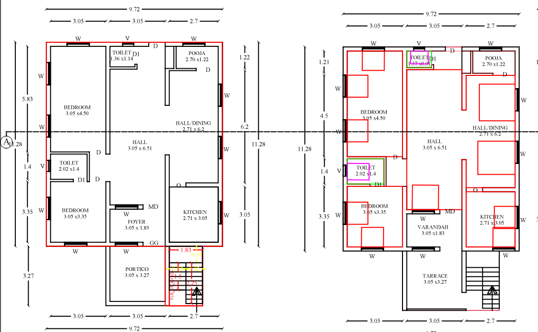
EXI. GROUND FLOOR PLAN
