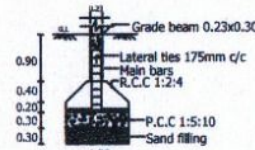
FOOTING DETAILS SCALE 1:50
