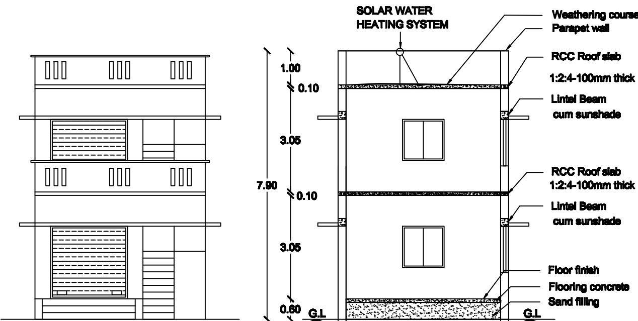
FRONT ELEVATION
