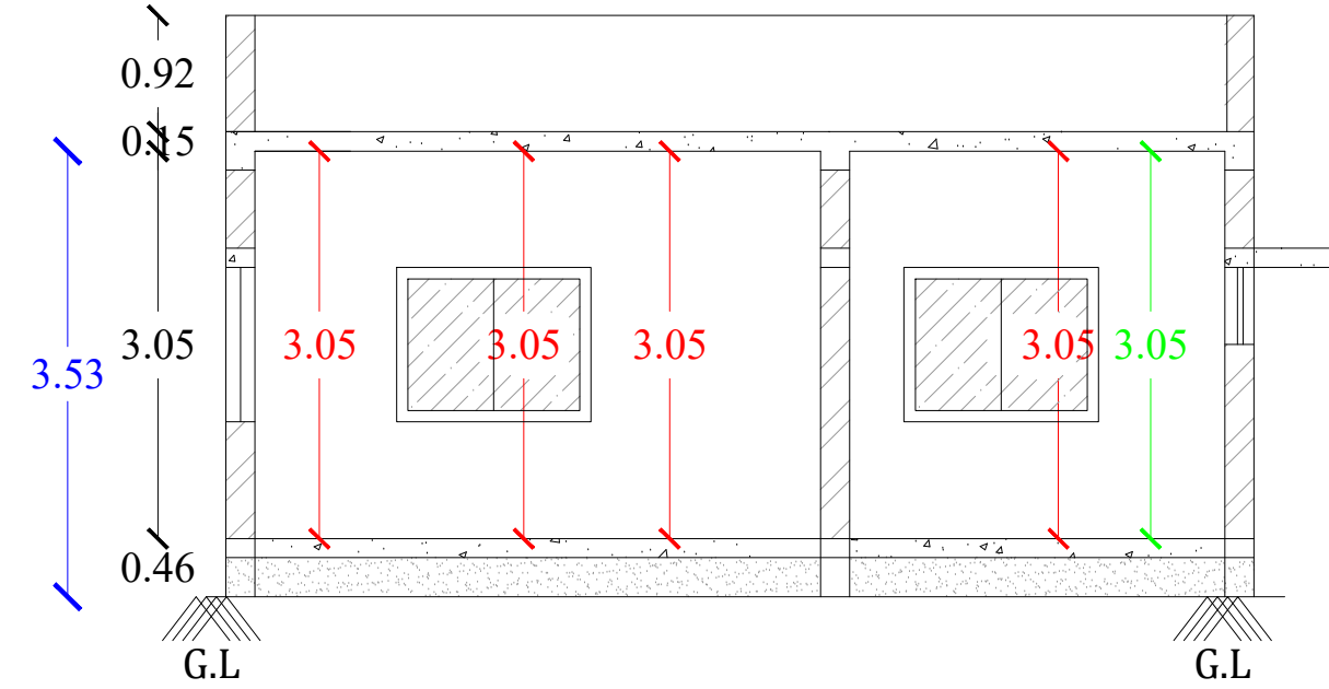
SECTION-AA
