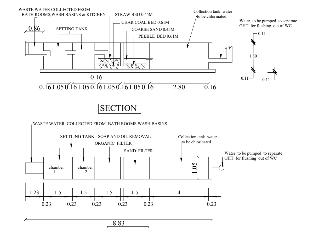
WASTE WATER RECYCLING SYSTEM
