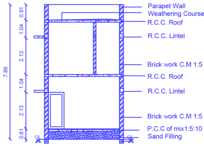
RS - CROSS SECTION
