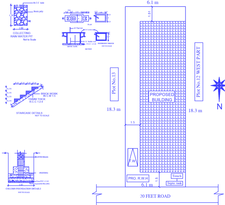
SITE PLAN (1:100)
