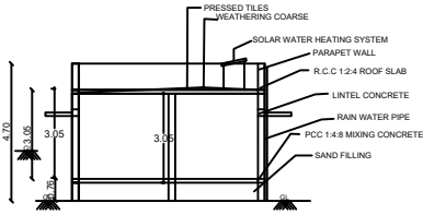
SECTION NO - "AA"
