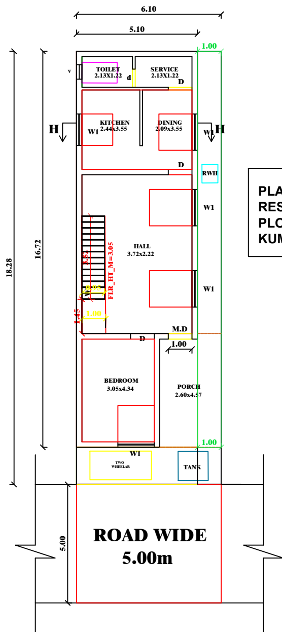
GROUND FLOOR CUM SITE PLAN
