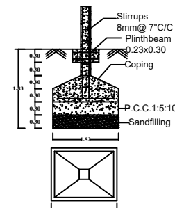
Foundation Details
