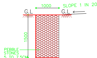
SECTION OF PEBBLE TRENCH SCALE : 1 : = 100
