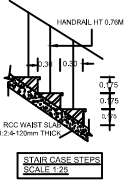
STAIR CASE STEPS
