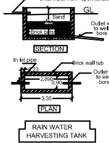
RAIN WATER HARVESTING TANK
