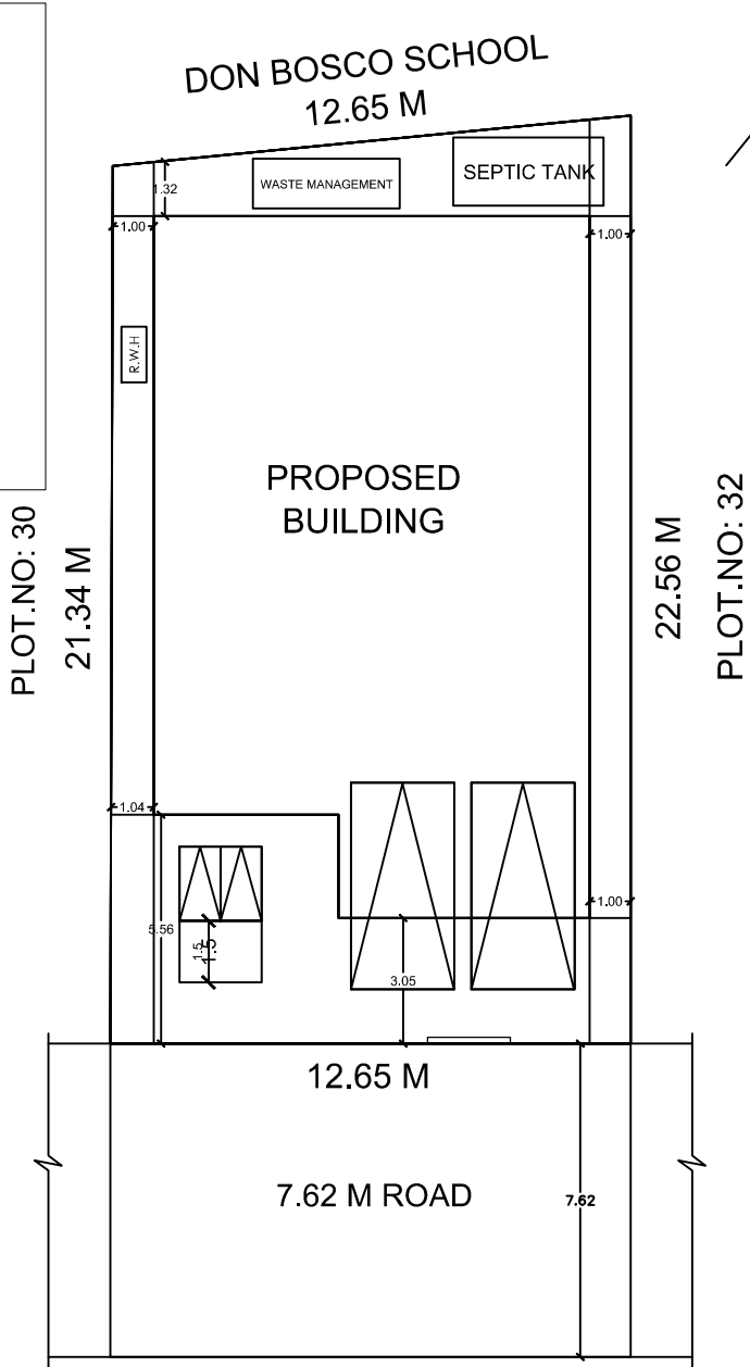
SITE PLAN
