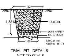
TRIAL PIT DETAILS
