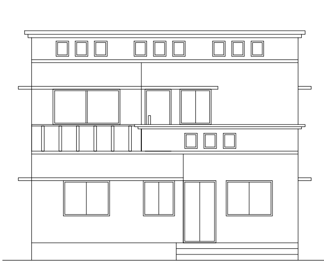
FRONT ELEVATION
