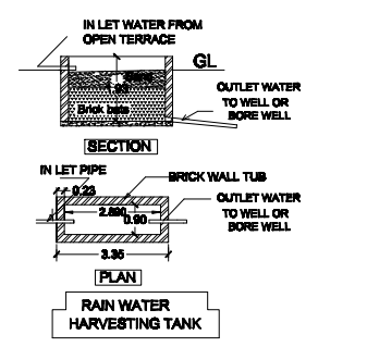
SCALE 1:50
