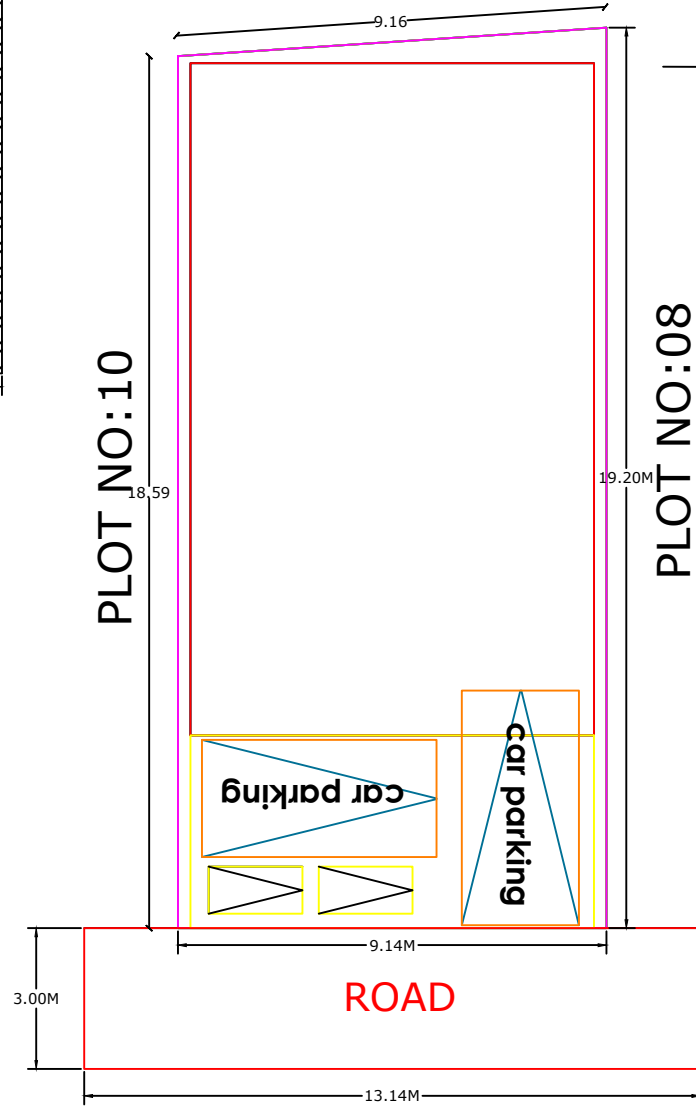
SITE PLAN
