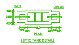
SEPTIC TANK DETAILS
