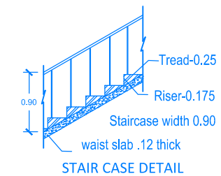
STAIR CASE DETAIL
