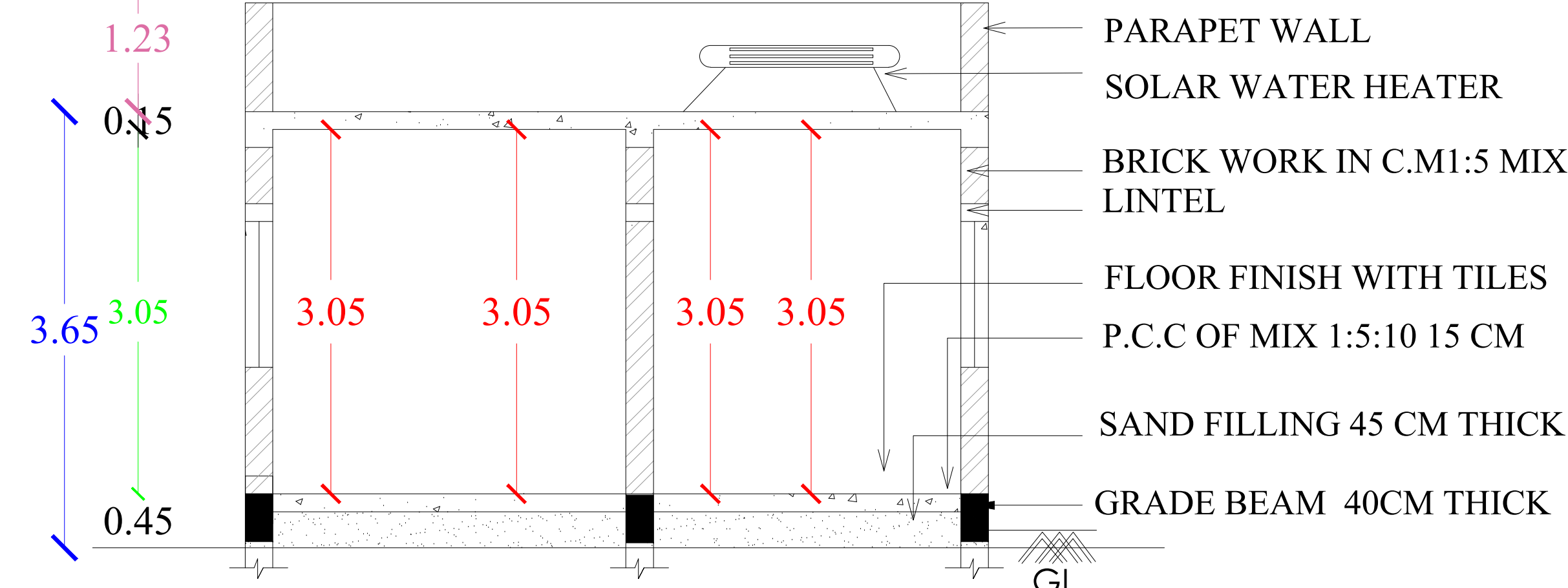
SECTION- AA
