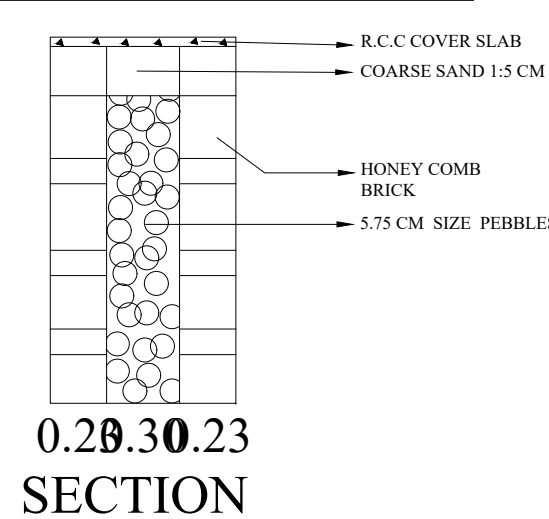
1.PERCOLATION PIT
