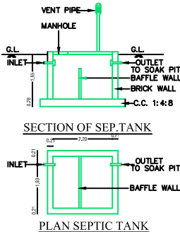
PLAN SEPTIC TANK
