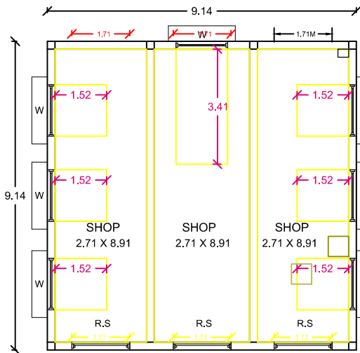
PRO. GROUND FLOOR
