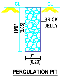
PERCULATION PIT
