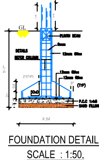
FOUNDATION DETAILS
