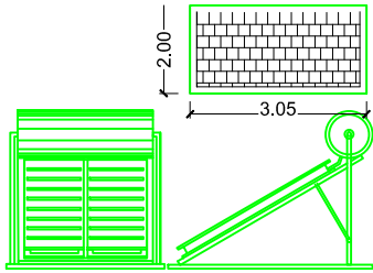
SOLAR PANEL
