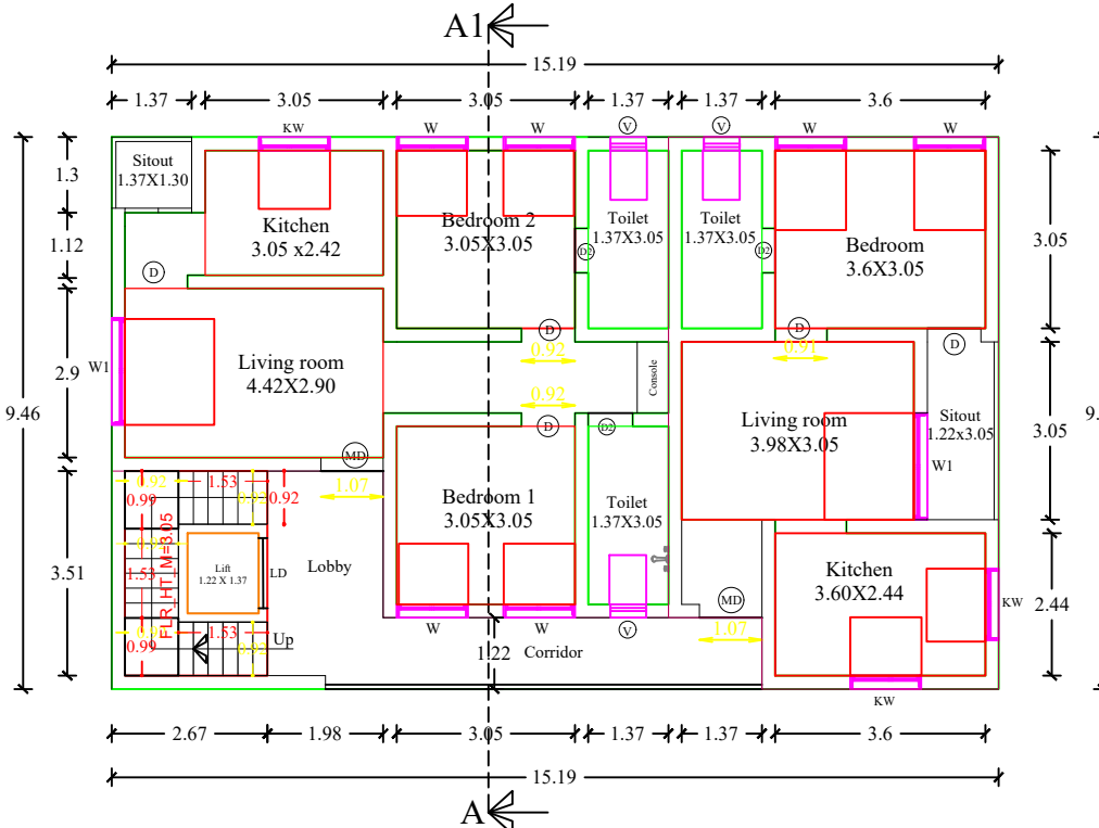
FIRST, SECOND & THIRD FLOOR PLAN TYPICAL_FLOOR_PLAN=1,2,3
