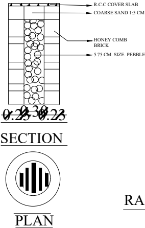
RAIN WATER HARVESTING 1.PERCOLATION PIT
