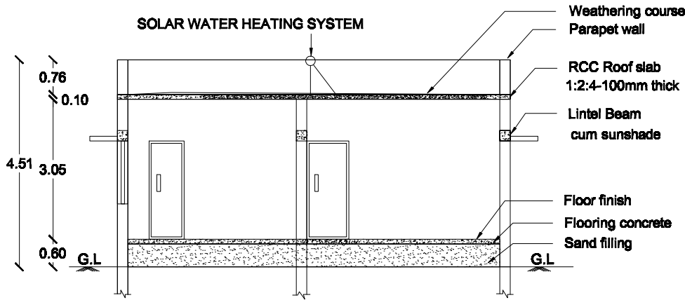
SECTION ON MK
