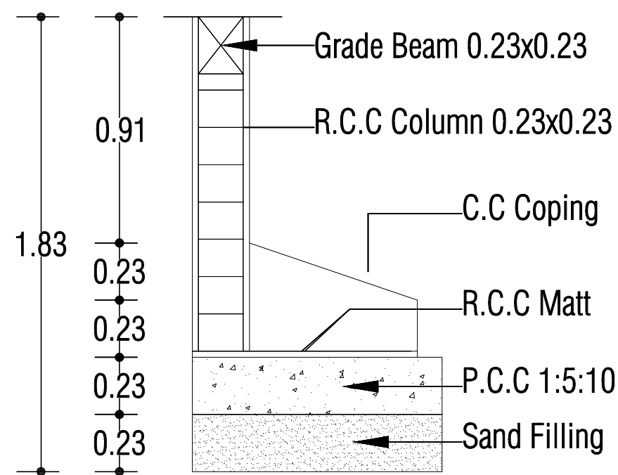
Foundation Details
