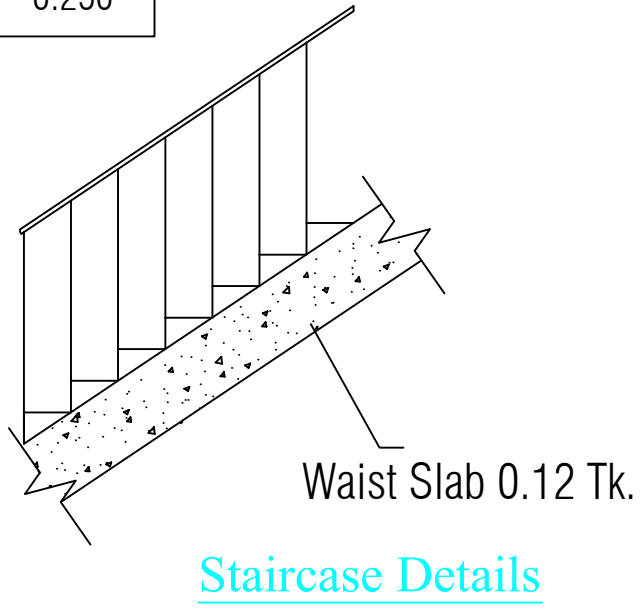
Staircase Details
