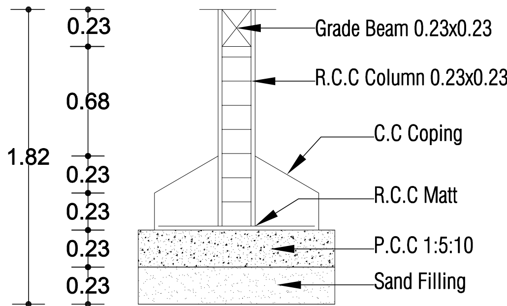
Foundation Detail
