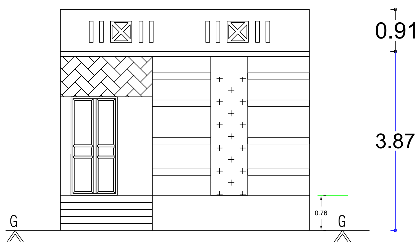
FRONT ELEVATION
